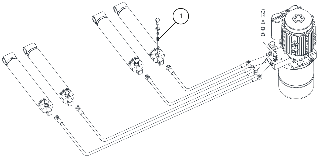
① Flow limiter
